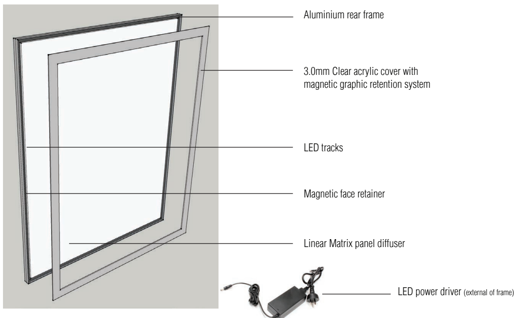
Magnetic peel out face
